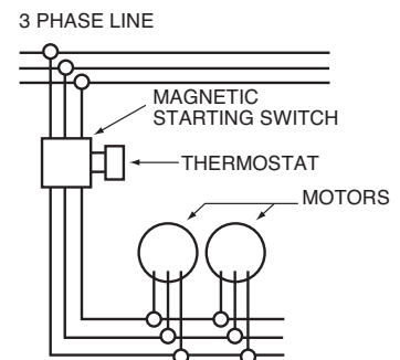
Figure 24 - THERMOSTATIC CONTROL OF SEVERAL THREE PHASE UNITS
