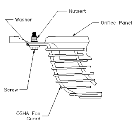
Figure 29 – OSHA Fan Guard
